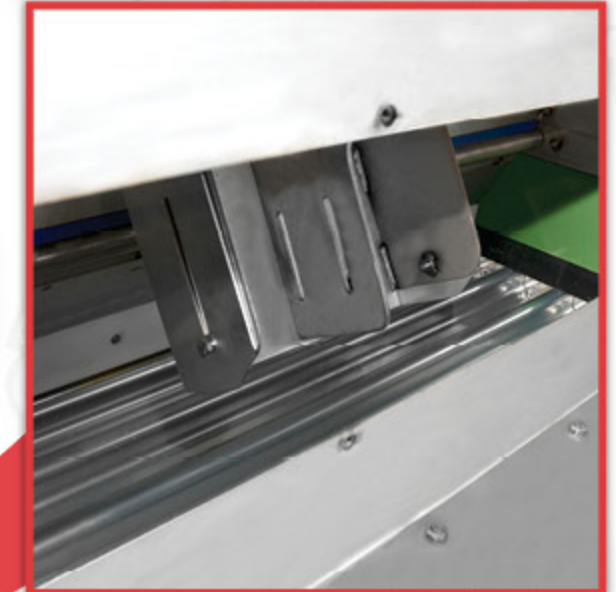
Oscillating feeder
